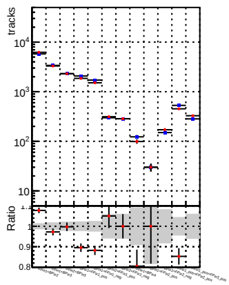
N of reco track vs. \chi^2 for \chi^2 < 10
