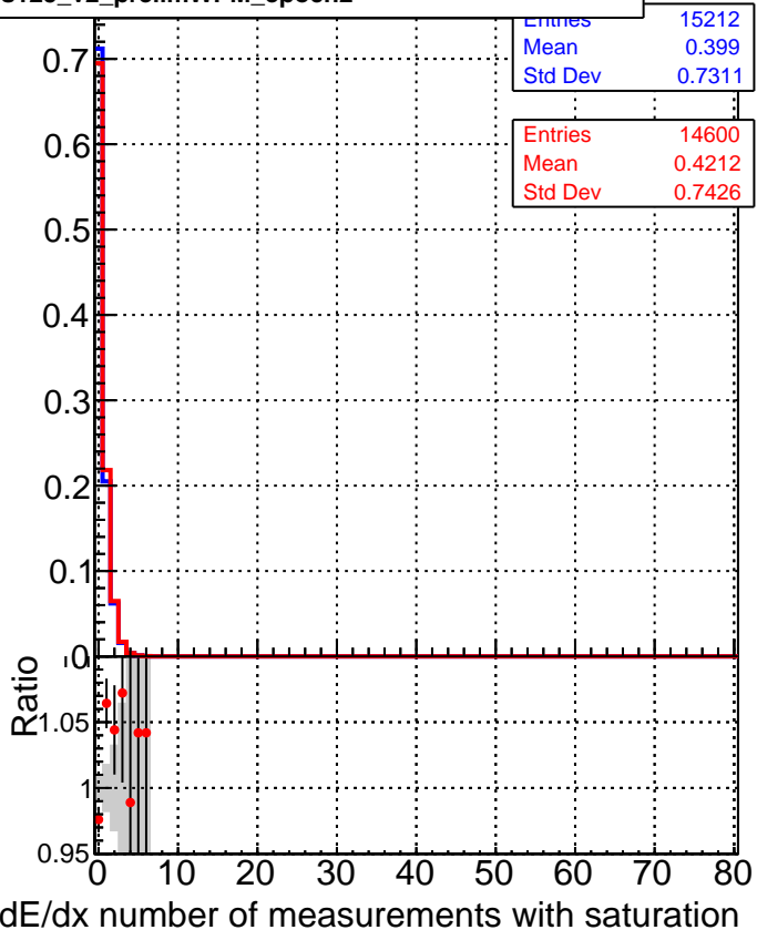
—●— DQM_CKF_XiMinusPU_retrainOldFiles125_v2_prelimWPM_epoch2
