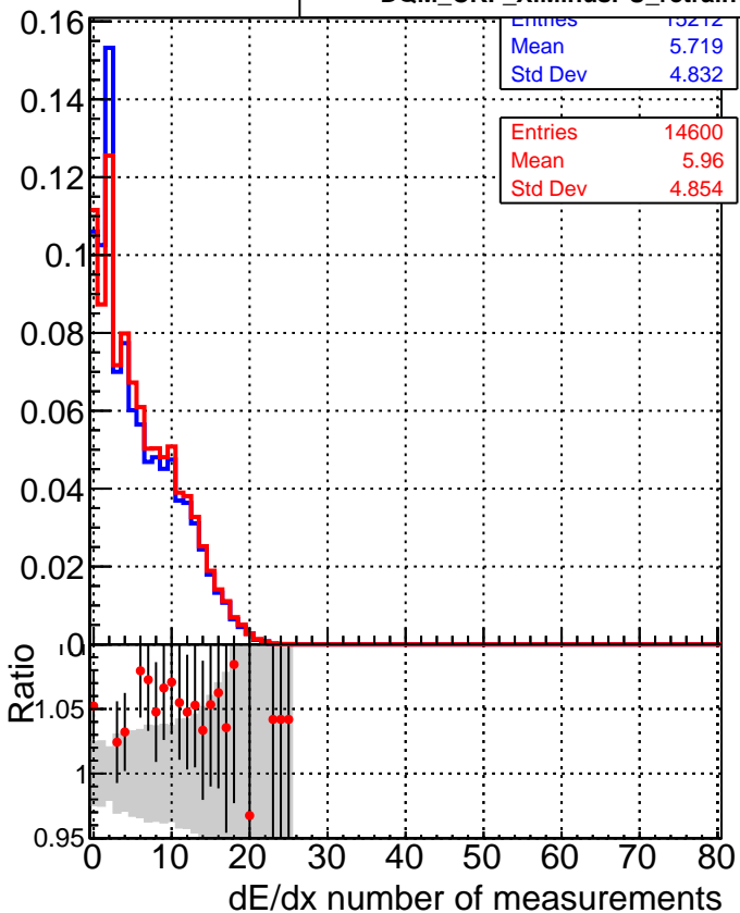
—●— DQM_CKF_XiMinusPU_retrainOldFiles125_v2_prelimWPM_epoch2
