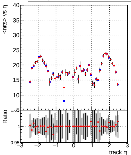
mean hits vs \eta Legend: DQM_CKF_XiMinusPU_base (blue line), DQM_CKF_XiMinusPU_retrainOldFiles125_v2_prelimWPM_epoch2 (red line)
