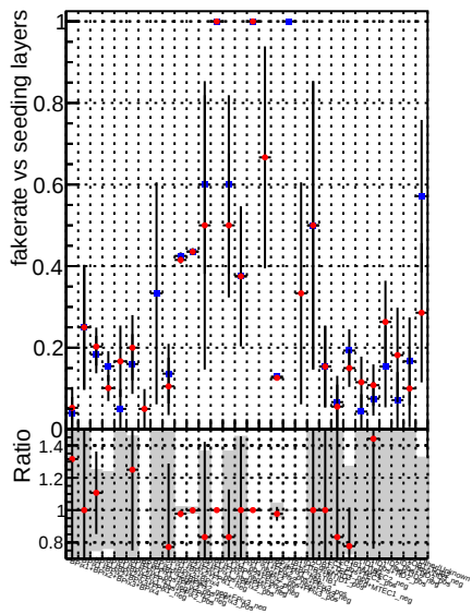
Fake rate vs. —•— DQM_CKF_XiMinusPU_base —•— DQM_CKF_XiMinusPU_retrainOldFiles125_v2_prelimWPM_epoch2
