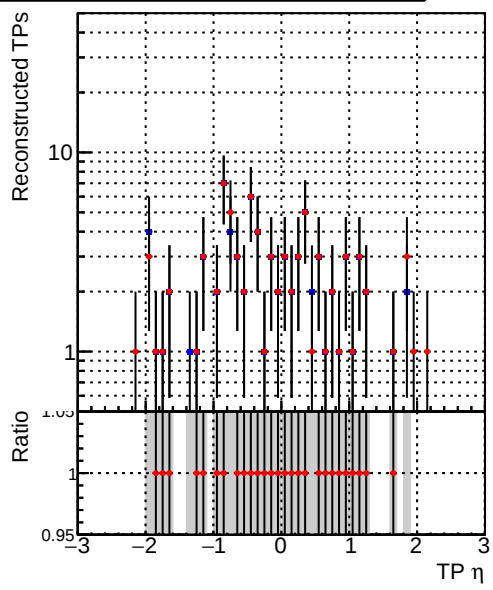
—•— DQM_CKF_XiMinusPU_base —•— DQM_CKF_XiMinusPU_retrainOldFiles125_v2_prelimWPM_epoch2
