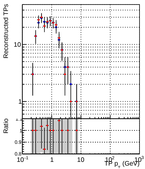
—•— DQM_CKF_XiMinusPU_base —•— DQM_CKF_XiMinusPU_retrainOldFiles125_v2_prelimWPM_epoch2
