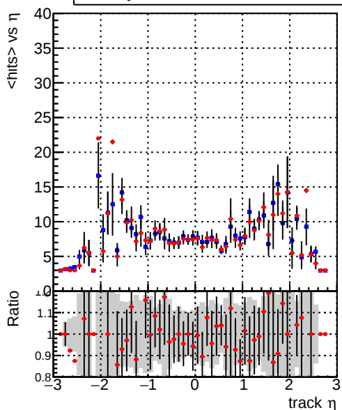
— DQM_CKF_XiMinusPU_base — DQM_CKF_XiMinusPU_retrainOldFiles125_v2_prelimWPM_epoch2 mean hits vs \eta
