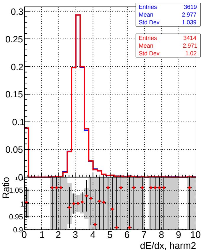
Legend: DQM_CKF_XiMinusPU_base (Blue line with squares) DQM_CKF_XiMinusPU_retrainOldFiles125_v2_prelimWPM_epoch2 (Red line with circles)
