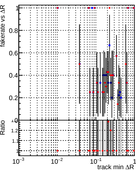
Legend: DQM_CKF_XiMinusPU_base (blue dots), DQM_CKF_XiMinusPU_retrainOldFiles125_v2_prelimWPM_epoch2 (red dots)
