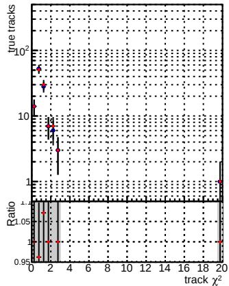
N of reco track vs. \chi^2 — DQM_CKF_XiMinusPU_base — DQM_CKF_XiMinusPU_retrainOldFiles125_v2_prelimWPM_epoch2
