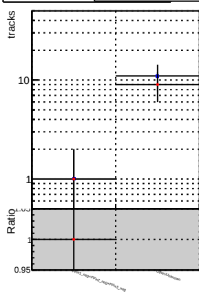
N of reco track vs. \chi^2 for DQM_CKF_XiMinusPU_base and DQM_CKF_XiMinusPU_retrainOldFiles125_v2_prelimWPM_epoch2
