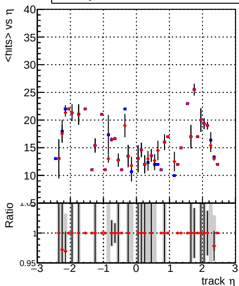
mean hit — DQM_CKF_XiMinusPU_base — DQM_CKF_XiMinusPU_retrainOldFiles125_v2_prelimWPM_epoch2
