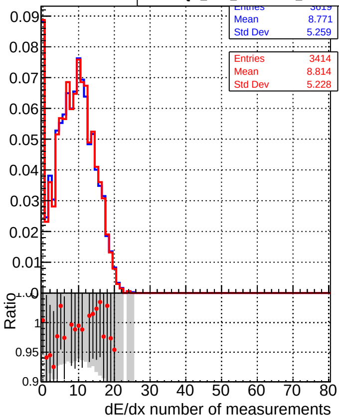
Legend for bottom row plots: ■ DQM_CKF_XiMinusPU_base ● DQM_CKF_XiMinusPU_retrainOldFiles125_v2_prelimWPM_epoch2
