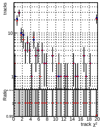
N of reco track vs. \chi^2 for DQM_CKF_XiMinusPU_base and DQM_CKF_XiMinusPU_retrainOldFiles125_v2_prelimWPM_epoch2
