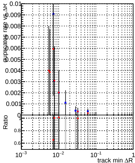
—•— DQM_CKF_XiMinusPU_base —•— DQM_CKF_XiMinusPU_retrainOldFiles125_v2_prelimWPM_epoch2
