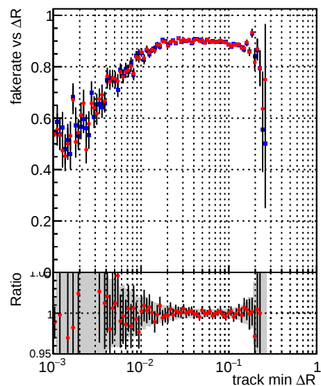
—•— DQM_CKF_XiMinusPU_base —•— DQM_CKF_XiMinusPU_retrainOldFiles125_v2_prelimWPM_epoch2
