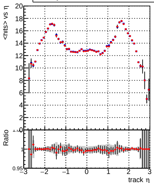
mean hits vs \eta — DQM_CKF_XiMinusPU_base — DQM_CKF_XiMinusPU_retrainOldFiles125_v2_prelimWPM_epoch2
