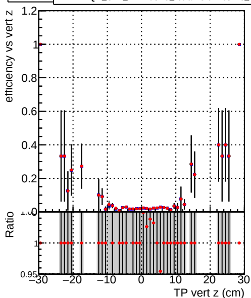
Efficiency vs. Sim. PV z —●— DQM_CKF_XiMinusPU_base —●— DQM_CKF_XiMinusPU_retrainOldFiles125_v2_prelimWPM_epoch2
