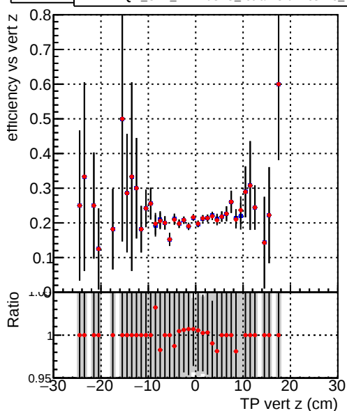
Efficiency vs. TP vert z (cm) —●— DQM_CKF_XiMinusPU_base —●— DQM_CKF_XiMinusPU_retrainOldFiles125_v2_prelimWPM_epoch2
