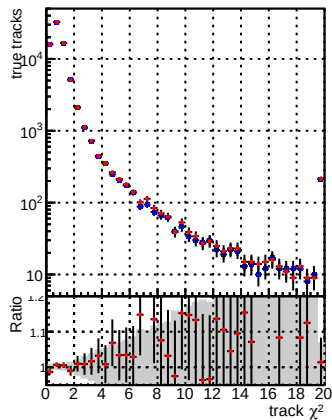
N of reco track vs. \chi^2 —●— DOM CKF XiMinusPU_base —●— DOM CKF XiMinusPU_retrainOldFiles125_v2_prelimWPM_epoch2
