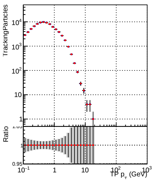
Legend: DQM_CKF_XiMinusPU_base (blue dots), DQM_CKF_XiMinusPU_retrainOldFiles125_v2_prelimWPM_epoch2 (red dots)
