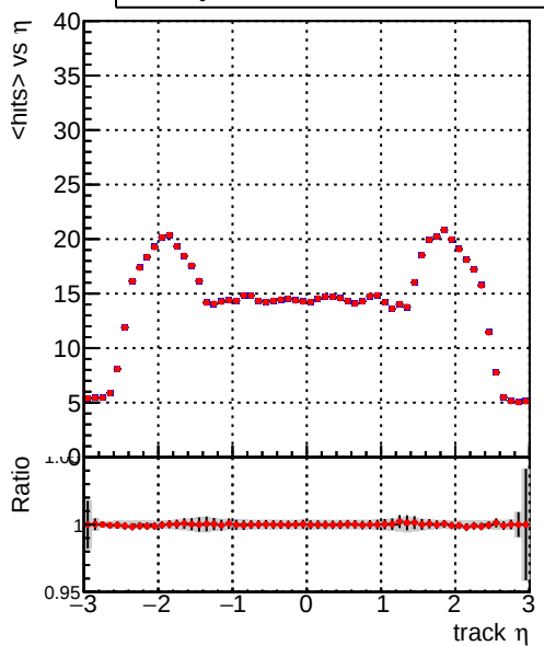
mean hits — DQM_CKF_XiMinusPU_base — DQM_CKF_XiMinusPU_retrainOldFiles125_v2_prelimWPM_epoch2
