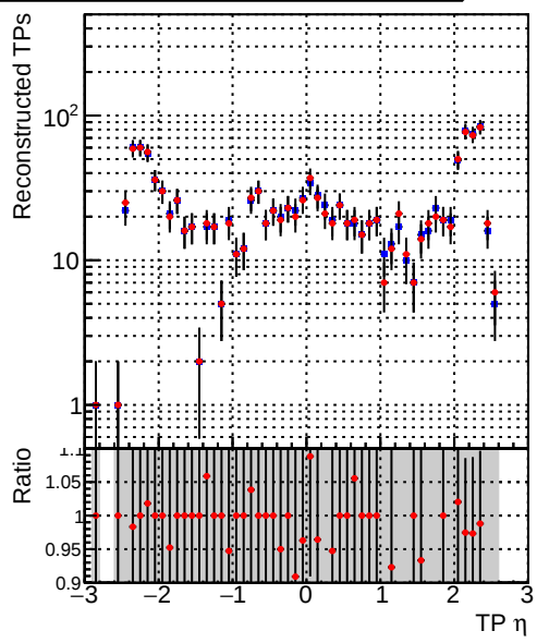
—•— DQM_CKF_XiMinusPU_base —•— DQM_CKF_XiMinusPU_retrainOldFiles125_v2_prelimWPM_epoch1
