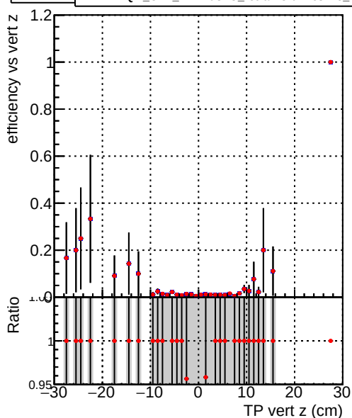
Efficiency vs. TP vert z (cm) —●— DQM_CKF_XiMinusPU_base —●— DQM_CKF_XiMinusPU_retrainOldFiles125_v2_prelimWPM_epoch1
