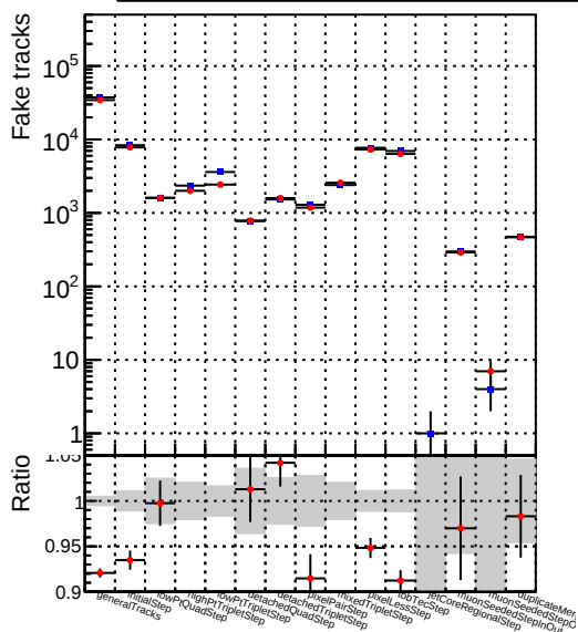
Number —●— DQM_CKF_XiMinusPU_retrainOldFiles125_v2_prelimWPM_epoch1
