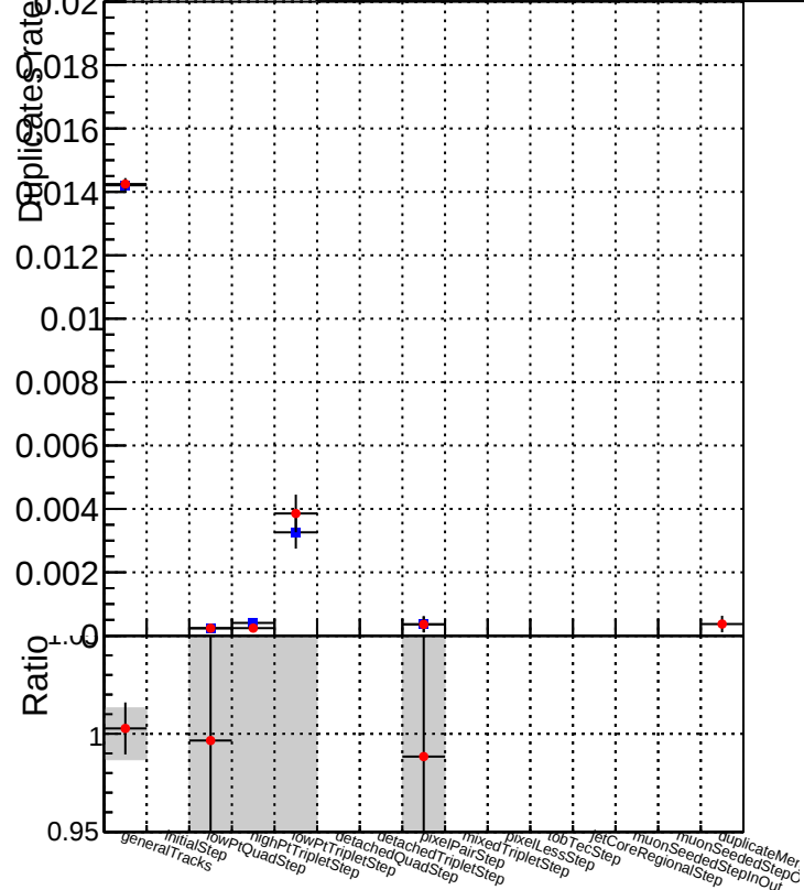
Duplicates rate vs collection Legend: DQM_CKF_XiMinusPU_base (blue square) DQM_CKF_XiMinusPU_retrainOldFiles125_v2_prelimWPM_epoch1 (red circle)
