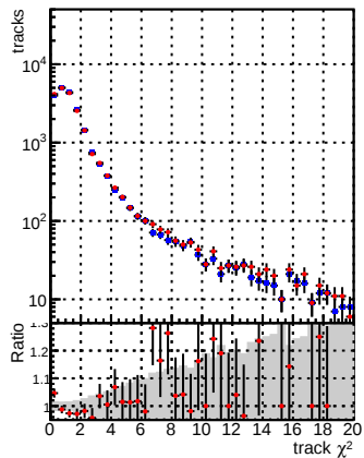
N of reco track vs. \chi^2 for DQM_CKF_XiMinusPU_base (blue circles) and DQM_CKF_XiMinusPU_retrainOldFiles125_v2_prelimWPM_epoch1 (red circles).
