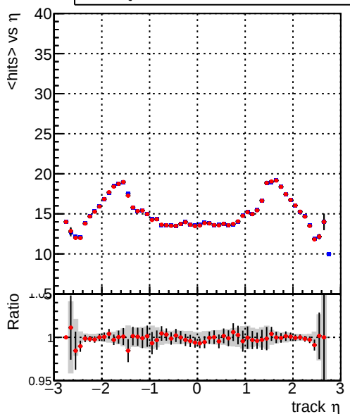
mean hits — DQM_CKF_XiMinusPU_base — DQM_CKF_XiMinusPU_retrainOldFiles125_v2_prelimWPM_epoch1
