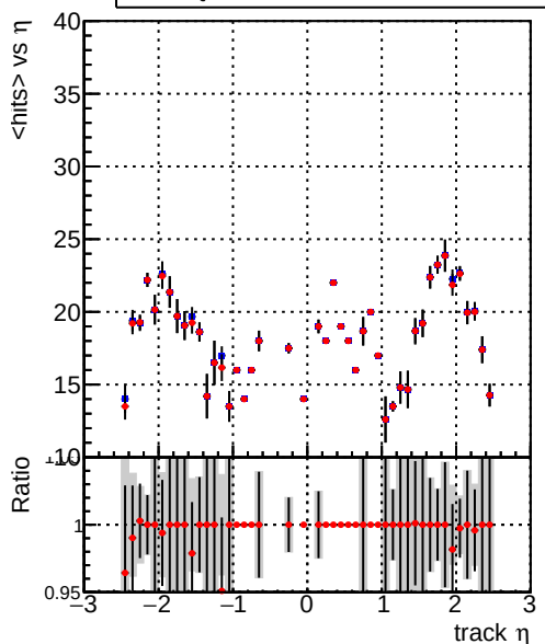
mean hits vs \eta Legend: DQM_CKF_XiMinusPU_base (blue line), DQM_CKF_XiMinusPU_retrainOldFiles125_v2_prelimWPM_epoch1 (red line)
