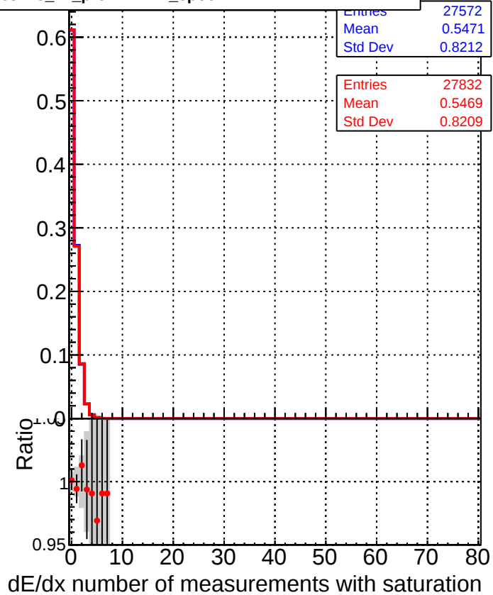
—■ DQM_CKF_XiMinusPU_base —● DQM_CKF_XiMinusPU_retrainOldFiles125_v2_prelimWPM_epoch1
