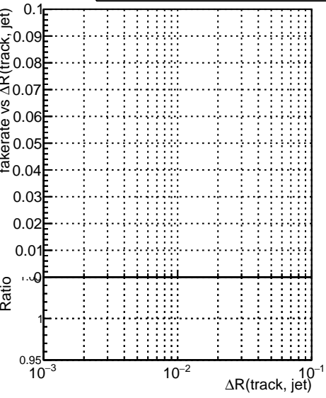
—●— DQM_CKF_XiMinusPU_base —●— DQM_CKF_XiMinusPU_retrainOldFiles125_v2_prelimWPM_epoch1
