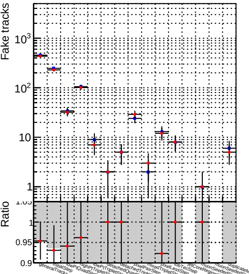
Number Model 1 DQM_CKF_XiMinusPU_retrainOldFiles125_v2_prelimWPM_epoch1
