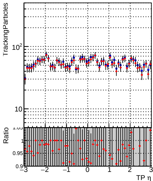
—■— DQM_CKF_XiMinusPU_base —●— DQM_CKF_XiMinusPU_retrainOldFiles125_v2_prelimWPM_epoch1
