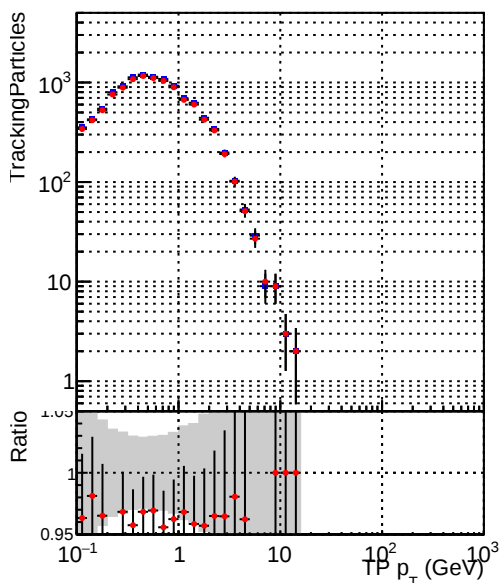
—■— DQM_CKF_XiMinusPU_base —●— DQM_CKF_XiMinusPU_retrainOldFiles125_v2_prelimWPM_epoch1
