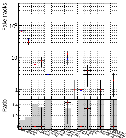
Number —●— DQM_CKF_XiMinusPU_retrainOldFiles125_v2_prelimWPM_epoch1
