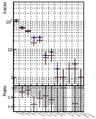
N of reco track vs. \chi^2 DQM_CKF_XiMinusPU_base DQM_CKF_XiMinusPU_retrainOldFiles125_v2_prelimWPM_epoch1
