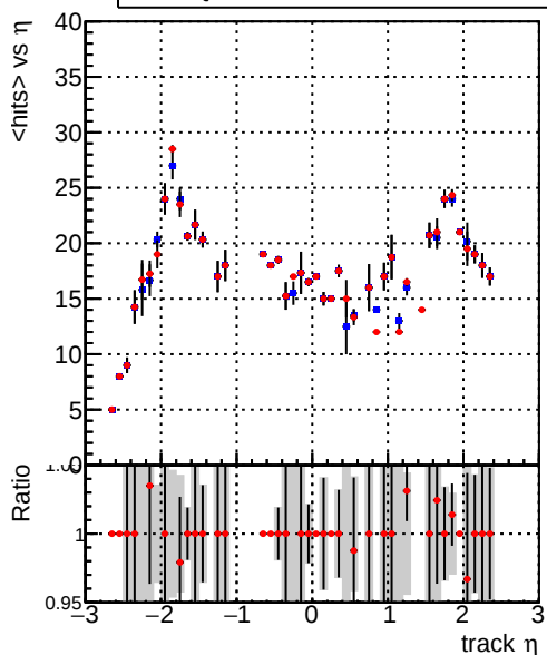
mean hit — DQM_CKF_XiMinusPU_base — DQM_CKF_XiMinusPU_retrainOldFiles125_v2_prelimWPM_epoch1
