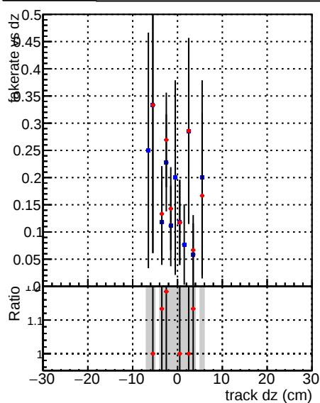
—●— DQM_CKF_XiMinusPU_base —●— DQM_CKF_XiMinusPU_retrainOldFiles125_v2_prelimWPM_epoch1
