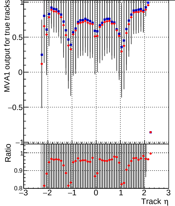
MVA1 of associated tracks (recoToSim) vs. track \eta Legend: ■ DQM_CKF_XiMinusPU_base ● DQM_CKF_XiMinusPU_retrainOldFiles125_v2_prelimWPM_epoch1
