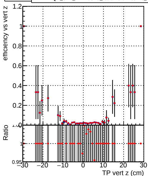
Efficiency vs. TP vert z —●— DQM_CKF_XiMinusPU_base —●— DQM_CKF_XiMinusPU_retrainOldFiles125_v2_prelimWPM_epoch1
