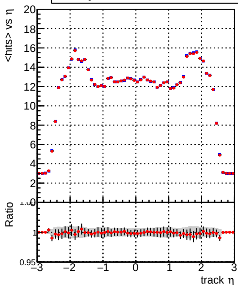
mean hits — DQM_CKF_XiMinusPU_base — DQM_CKF_XiMinusPU_retrainOldFiles125_v2_prelimWPM_epoch1
