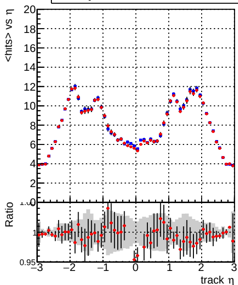
mean hits vs \eta Legend: DQM_CKF_XiMinusPU_base (blue line), DQM_CKF_XiMinusPU_retrainOldFiles125_v2_prelimWPM_epoch1 (red line)
