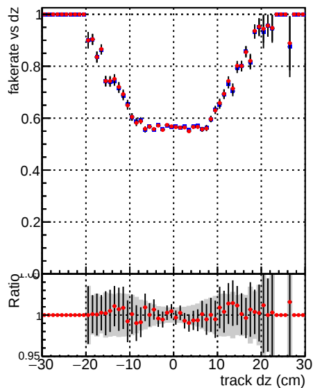
Fake rate vs dz DQM CKF_XiMinusPU_base DQM CKF_XiMinusPU_retrainOldFiles125_v2_prelimWPM_epoch1
