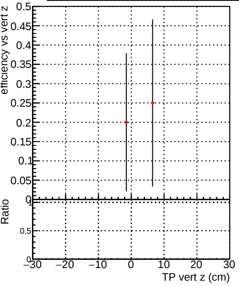
Efficiency vs TP vert z (cm) Legend: DQM_CKF_XiMinusPU_base DQM_CKF_XiMinusPU_retrainOldFiles125_v2_prelimWPM_epoch1
