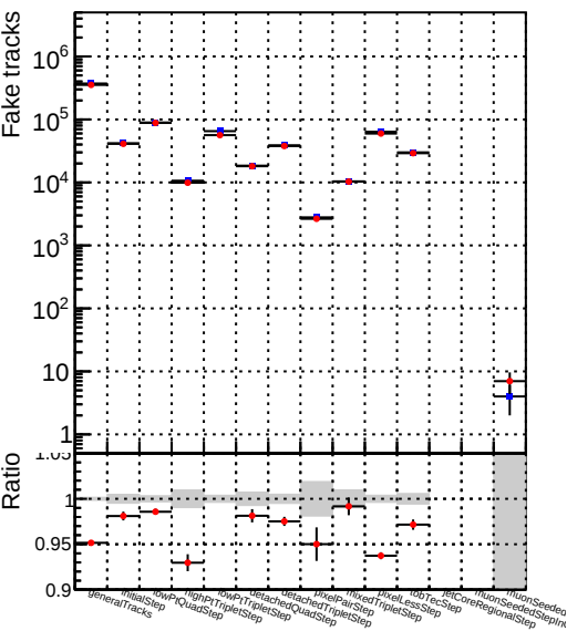
Numbe 1 DQM_CKF_XiMinusPU_retrainOldFiles125_v2_prelimWPM_epoch1
