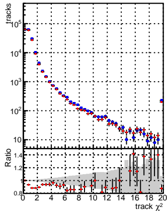
N of reco track vs. s DQM_CKF_XiMinusPU_base DQM_CKF_XiMinusPU_retrainOldFiles125_v2_prelimWPM_epoch1
