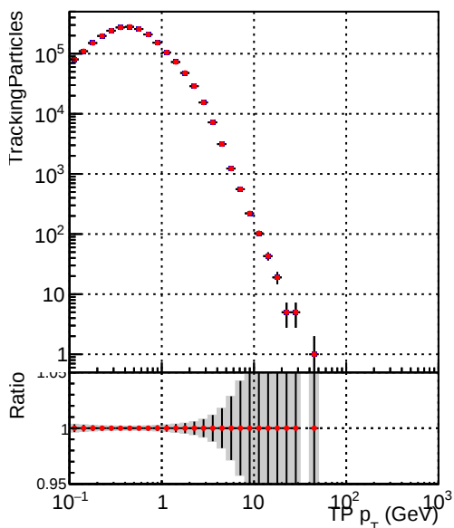
—•— DQM_CKF_XiMinusPU_base —•— DQM_CKF_XiMinusPU_retrainOldFiles125_v2_prelimWPM_epoch1
