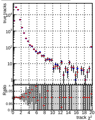
N of reco track vs. —●— DQM_CKF_XiMinusPU_base —●— DQM_CKF_XiMinusPU_retrainOldFiles125_v2_prelimWPM_epoch1
