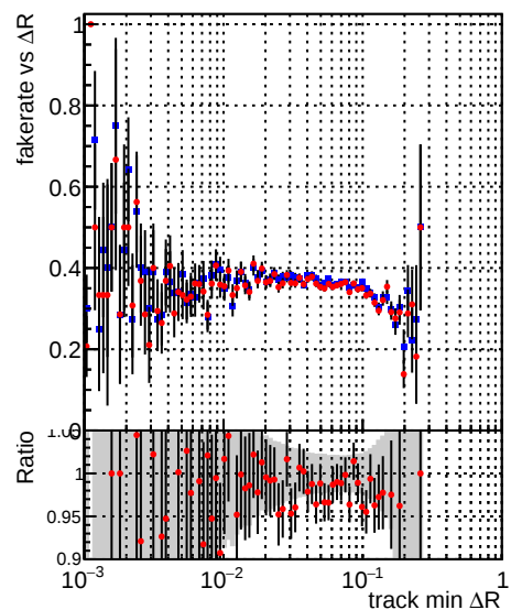
Legend: - DQM_CKF_XiMinusPU_base (blue line with error bars) - DQM_CKF_XiMinusPU_retrainOldFiles125_v2_prelimWPM_epoch1 (red line with error bars)
