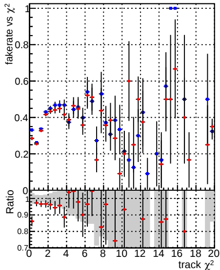
Fake rate vs. —■— DQM CKF_XiMinusPU_base —●— DQM CKF_XiMinusPU_retrainOldFiles125_v2_prelimWPM_epoch1
