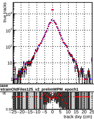
N of associated (recoToSim) tracks vs dxy
