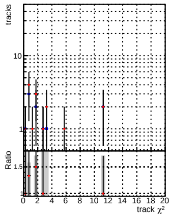
N of reco track vs. \chi^2 for DQM CKF XiMinusPU_base and DQM CKF XiMinusPU_retrainOldFiles125_v2_prelimWPM_epoch1
