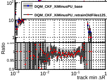
N of reconstructed tracks vs dR(track,jet)
